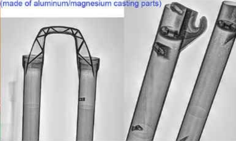
Unicomp X-Ray Inspect Bicycle Front Fork (made of aluminum/magnesium casting parts)
